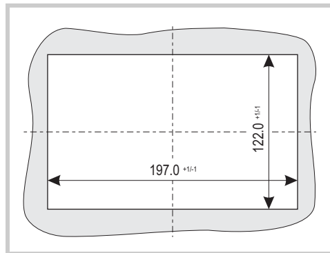
Fig.. 30 Mounting cutout for 7.0" devices
