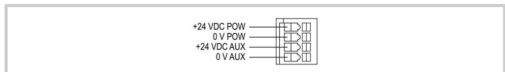
Fig.. 20 WAGO plug connector (view from wiring side)
