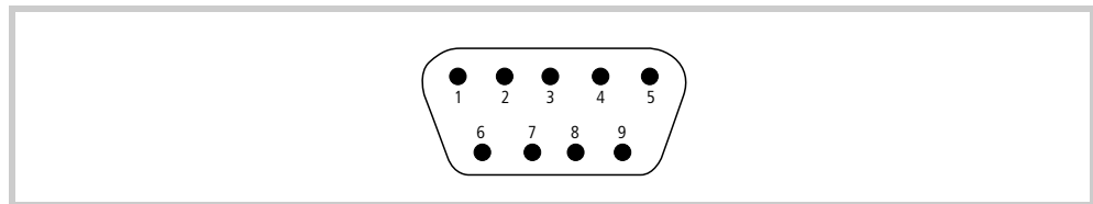
Fig.. 26 RS485 interface (9-pin, D-Sub, male, UNC)
