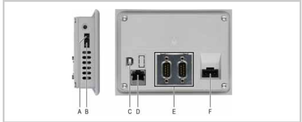
Fig.. 7 Example Interfaces of the 3.5" devices without Smart WireDT master
