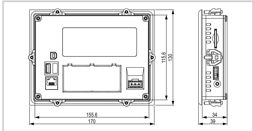
Fig.. 41 Mechanical dimensions of the 5.7" devices in mm
