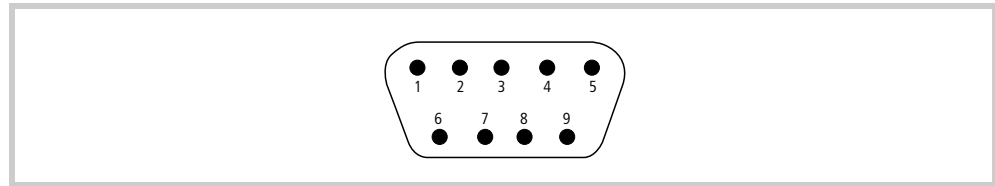
Fig.. 14 RS232 interface (9-pin, D-Sub, male, UNC)
