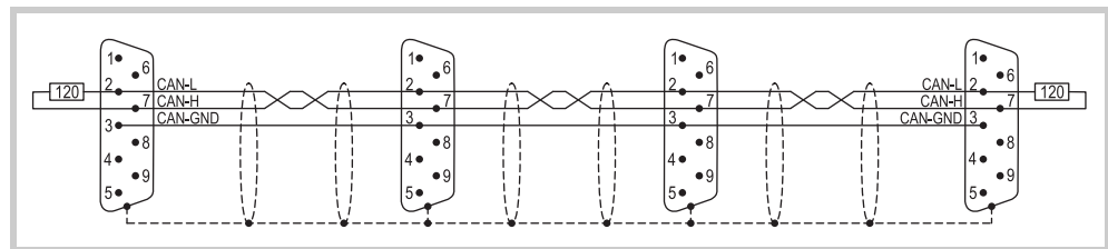
Fig.. 23 Bus segment with four nodes
