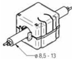
Fig.. 38 Screening with snap-together ferrite ring
