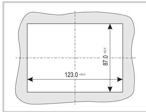
Fig.. 28 Mounting cutout for 3.5" devices
