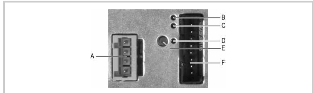
Fig.. 18 SmartWire-DT master interface
