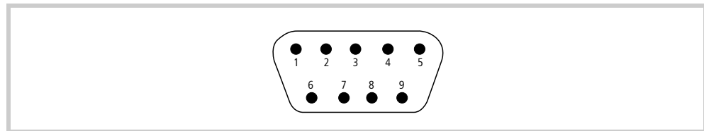
Fig.. 22 CAN interface (9-pin, D-Sub, male, UNC)
