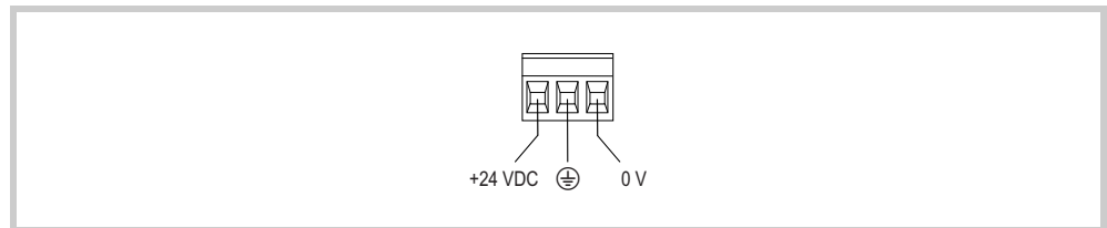
Fig.. 12 Phoenix Contact MSTB 2.5/3-ST-5.08 plug connector (view from wiring side)
