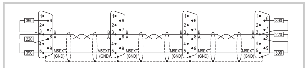
Fig.. 25 Bus segment with four nodes
