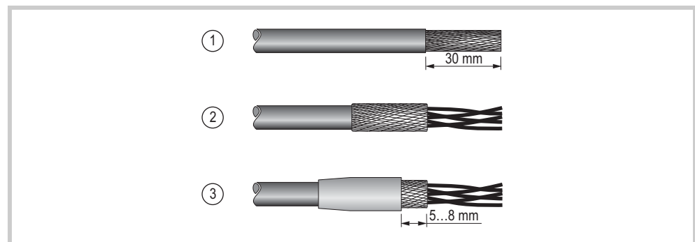
Fig.. 9 Connecting the cable screen
