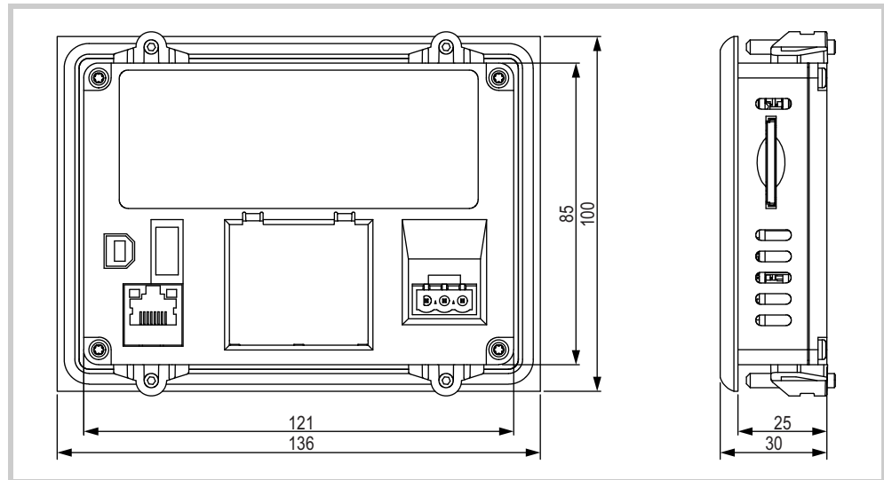
Fig.. 40 Mechanical dimensions of the 3.5" devices in mm
