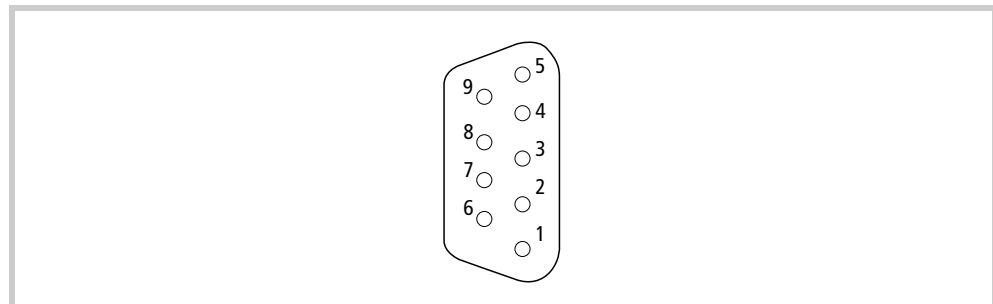
Fig.. 24 Profibus interface (9-pin, D-Sub, female, UNC)
