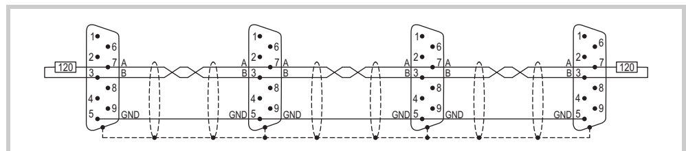
Fig.. 27 Bus segment with four nodes
