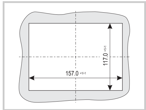
Fig.. 29 Mounting cutout for 5.7" devices
