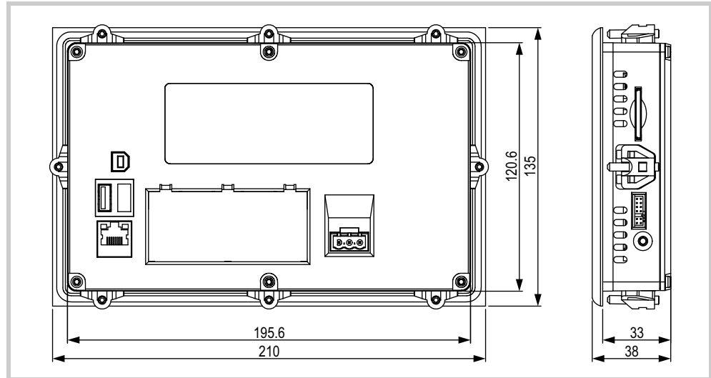
Fig.. 42 Mechanical dimensions of the 7.0" devices in mm
